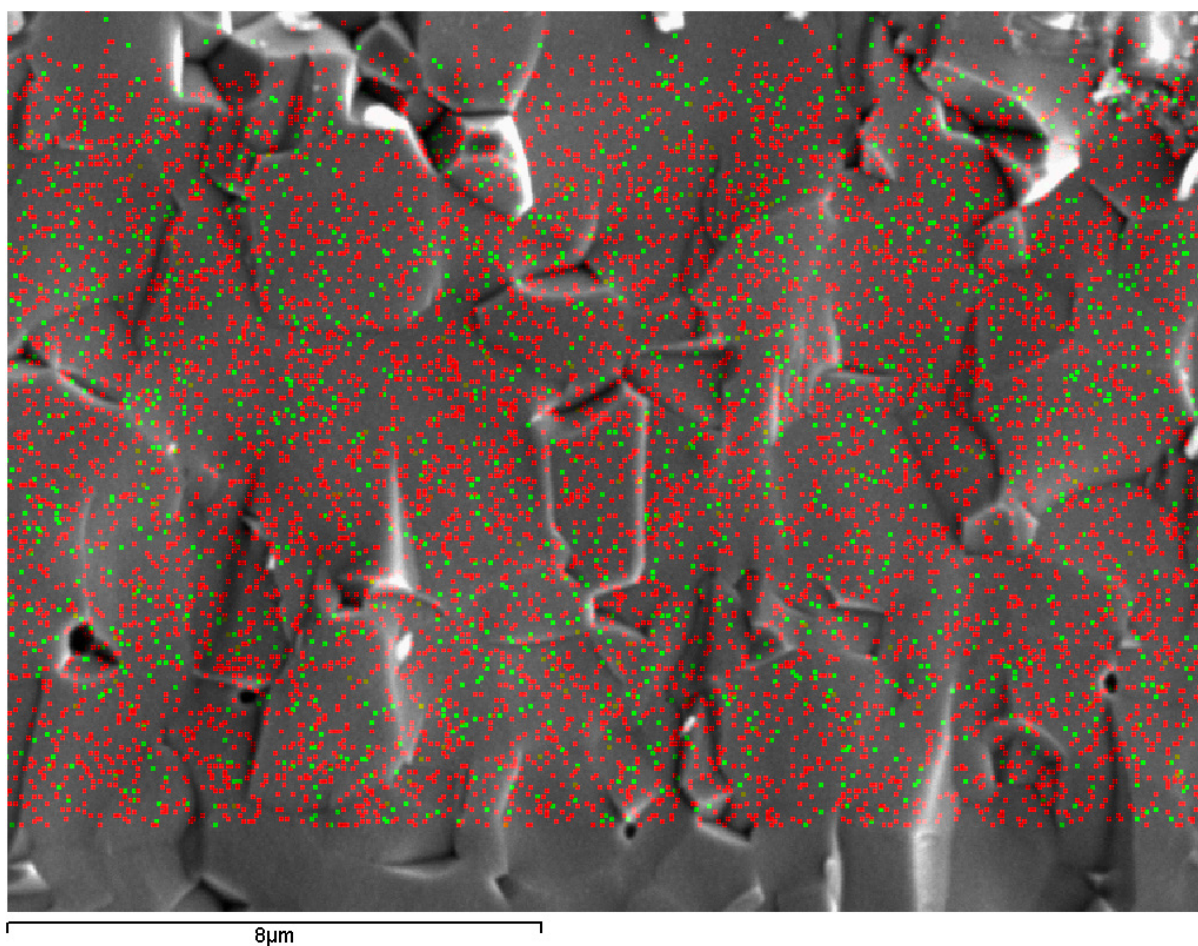
Figure S1 EDX mapping for Si-substituted hydroxyapatite bioceramics (Red dots – phosphorous, green dots – silicon).
