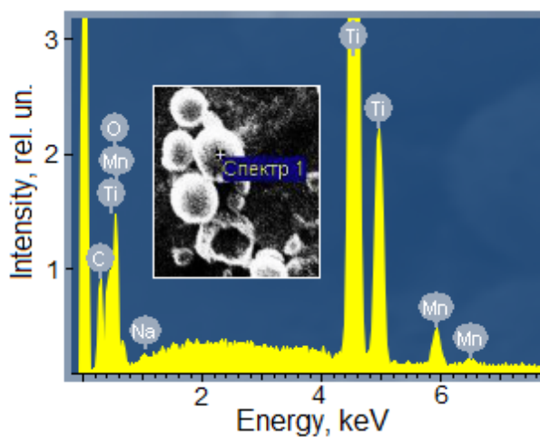
Figure S1. EDX spectrum of nanoparticles forming the microcapsule walls.
