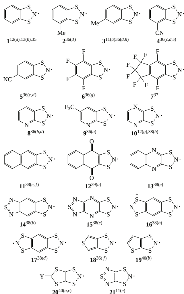
Scheme 2 Selected WRs and related fused 1,3,2-dithiazolyli, Y = O, S, (NC) 2 C; (see refs. 18 and 41 for other hydrocarbon WRs and ref. 37 for fluorocarbon WRs).
