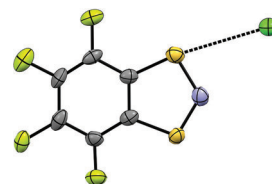
Figure 2 XRD structure of [\mathbf{6}]^+[\text{Cl}]^- 36(g),37 (CCDC 731911). Colour code: C, grey; Cl, green; F, light green; N, blue; S, yellow; dashed line indicates \text{S}\cdots\text{Cl}^- shortened contact (here and below, as compared with the sum of the corresponding van der Waals (VdW) radii, i.e. , SBI/ChB; see discussion below).
