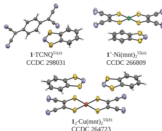
Figure 4 XRD molecular structures of WRs' complexes, coordination compounds and salts. Colour code: C, grey; H, light grey; Cu, red; N, blue; Ni, green; S, yellow.
