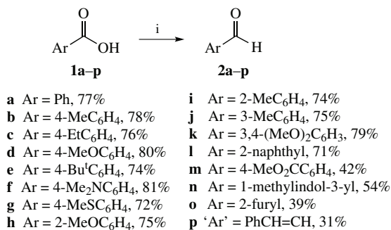
Scheme 1 Reagents and optimized conditions: i , 1 (0.2 mmol), NiBr 2 ·3H 2 O (20 mol%), dtbbpy (20 mol%), Zn (20 mol%), Ph 2 SiH 2 (2.25 equiv.), (MeO) 2 C 2 O 3 (2 equiv.), 2,6-lutidine (1.2 equiv.), EtOAc (4 ml), 60 °C, 24 h, GC yields. For Ar = 4-F 3 CC 6 H 4 , 4-O 2 NC 6 H 4 and 3-pyridyl, trace yields; for Ar = 4-BrC 6 H 4 , product mixture was formed.
