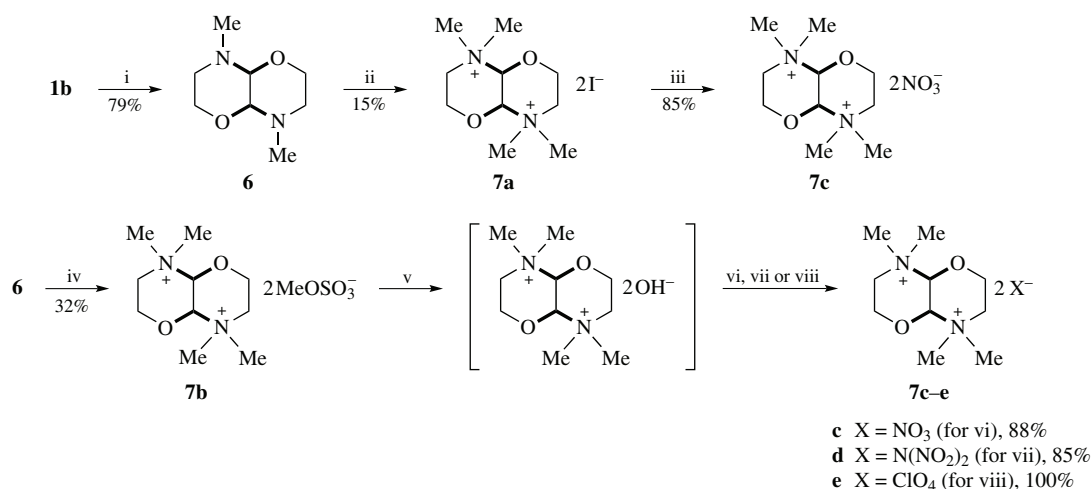
Scheme 3 Reagents and conditions: i, (CHOCHO) 3 ·2H 2 O, 40 °C, 3 h; ii, MeI, MeOH, 40 °C, 10 h; iii, Pb(NO 3 ) 2 , H 2 O, room temperature, 30 min; iv, (MeO) 2 SO 2 , MeCN, 80 °C, 4 h; v, NaOH, EtOH, H 2 O, THF, –10 °C, 30 min; vi, NH 4 NO 3 , H 2 O, room temperature, 20 min; vii, NH 4 N(NO 2 ) 2 , H 2 O, room temperature, 20 min; viii, NH 4 ClO 4 , H 2 O, room temperature, 20 min.
