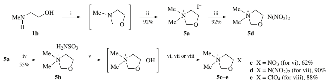
Scheme 2 Reagents and conditions: i, (CH 2 O) x , 40 °C, 3 h; ii, MeI, MeCN, room temperature, 20 h; iii, AgN(NO 2 ) 2 , H 2 O, room temperature, 30 min; iv, Pb(H 2 NSO 3 ) 2 , H 2 O, room temperature, 30 min; v, NaOH, EtOH, THF, 0 °C, 40 min; vi, NH 4 NO 3 , H 2 O, room temperature, 20 min; vii, NH 4 N(NO 2 ) 2 , H 2 O, room temperature, 20 min; viii, NH 4 ClO 4 , H 2 O, room temperature, 20 min.
