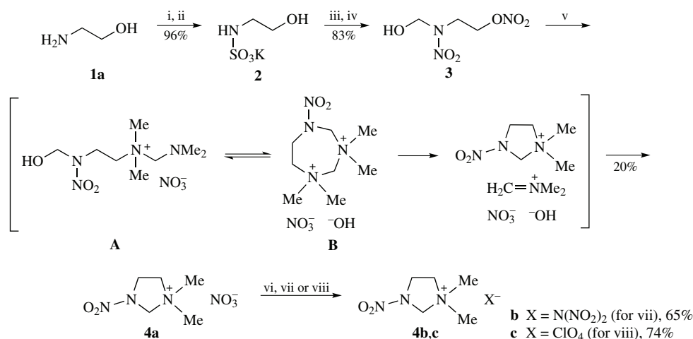
Scheme 1 Reagents and conditions: i, H 2 NSO 3 H, 178 °C, 9 h; ii, KOH, EtOH, room temperature, 40 min; iii, (CH 2 O) x , AcOH, room temperature, 20 min; iv, HNO 3 /H 2 SO 4 , –15 °C, 1 h; v, CH 2 (NMe 2 ) 2 , MeCN, 45 °C, 30 min; vi, Dowex 2 × 8 (OH – )/H 2 O, room temperature, 1.5 h; vii, NH 4 N(NO 2 ) 2 , H 2 O, room temperature, 20 min; viii, NH 4 ClO 4 , H 2 O, room temperature, 20 min.
