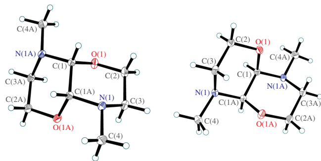
Figure 1 Molecular structure of isomeric (4aR*,8aR*)-4,8-dimethylperhydro[1,4]oxazino[3,2-b][1,4]oxazine 6 .
