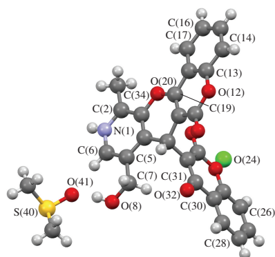
Figure 1 Molecular structure of compound 5 .
