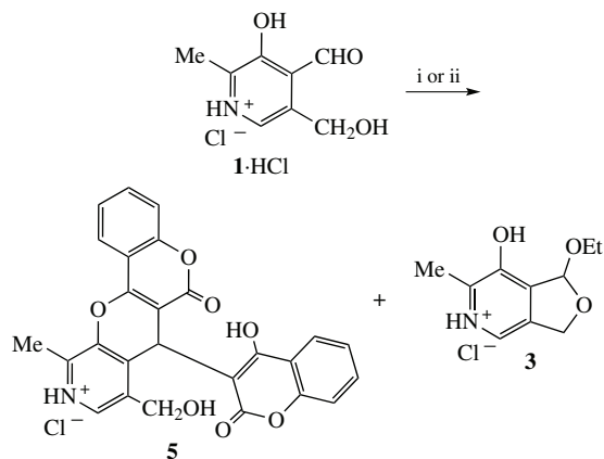
Scheme 2 Reagents and conditions: i, 2 (1 equiv.), EtOH (abs.), 78 °C, 10 h, yield of 5 46%, yield of 3 54%; ii, 2 (2 equiv.), EtOH (abs.), 78 °C, 10 h, yield of 5 67%, 3 is not formed.
