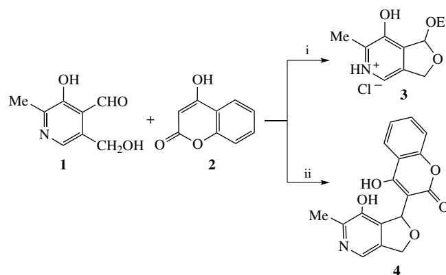
Scheme 1 Reagents and conditions: i, 2 (1 equiv.), EtOH (abs.)/HCl, reflux, 10 h; ii, 2 (1 equiv.), EtOH (abs.), reflux, 10 h, yield of 4 97%.
