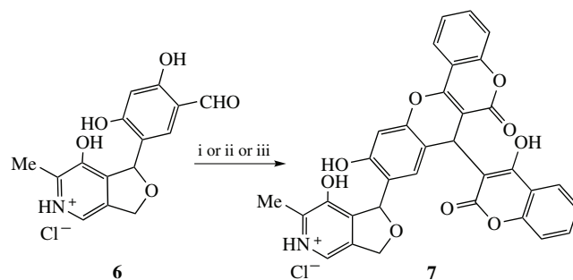
Scheme 3 Reagents and conditions: i, 2 (2 equiv.), EtOH (abs.), TsOH (cat.), 78 °C, 3 h, 98%; ii, 2 (2 equiv.), EtOH (abs.), without catalyst, 78 °C, 3 h, 90%; iii, 2 (2 equiv.), EtOH (abs.), piperidine (cat.), 78 °C, 3 h, 86%.
