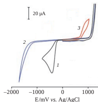
Figure 1 Cyclic voltammetric curves of (1) nitro compound 1a , (2) a product of its reductive heterocyclization 2a and (3) amino derivative 3 ; 5 \times 10^{-3} M in 8% HCl, glassy carbon working electrode ( d = 1.7 mm), potential sweep rate of 100 mV s -1 , T = 298 K.
