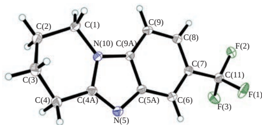
Figure 2 Molecular structure of 2a ( p = 50\% ). The disordering of the \text{CF}_3 group is not shown.
