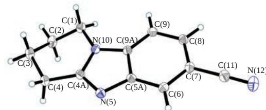
Figure 3 Molecular structure of 2c ( p = 50\% ). The disordering of the C(2) and C(3) atoms is not shown.
