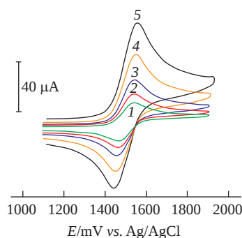
Figure 2 Cyclic voltammograms of 3 \times 10^{-3} M 1,1'-diphenyl-bis-germatrane 1 at a GC disc electrode (1.7 mm) in 0.1 M Bu 4 NPF 6 /MeCN at scan rates of (1) 0.05, (2) 0.1, (3) 0.2, (4) 0.5 and (5) 1.0 V s -1 . Temperature 298 K.
