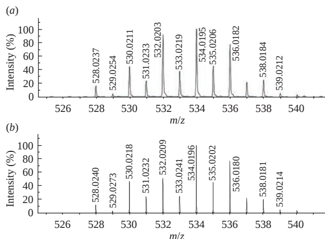
Figure 1 HRMS (ESI-MS) spectrum of 1,1'-diphenyl-bis-germatrane 1 (the molecular ion formation upon H + -ionization): (a) experimental and (b) calculated.
