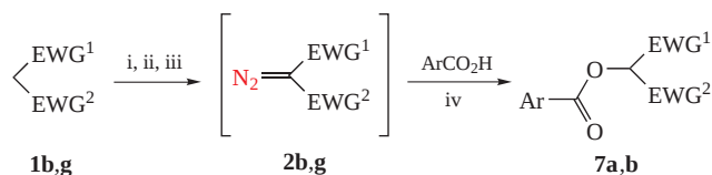
Scheme 2 Reagents and conditions: i, MsCl (1.1 equiv.), NaN_3 (1.2 equiv.), H_2O , room temperature, 10 min; ii, K_2CO_3 (0.6 equiv.), H_2O , room temperature, 60 min; iii, K_2CO_3 (1.0 equiv.), H_2O , room temperature, 3 h.
