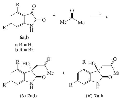
Scheme 1 Reagents and conditions: i, catalyst 1–5 , solvent, H 2 O (2 equiv.), room temperature, 24–180 h.
