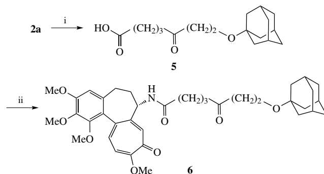
Scheme 2 Reagents and conditions: i, glutaric anhydride, 4-DMAP, CH 2 Cl 2 , room temperature, 24 h; ii, N -deacetylcolchicine, EEDQ, CH 2 Cl 2 , room temperature, 12 h.
