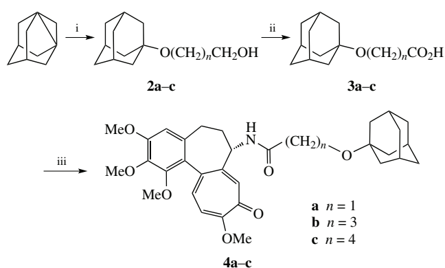
Scheme 1 Reagents and conditions: i, alkanediol, Et 2 O, 30–40 °C, 2–3 h; 13 ii, Jones reagent, THF, room temperature, 5 min; iii, N -deacetylcolchicine, EEDQ, CH 2 Cl 2 , room temperature, 12 h.
