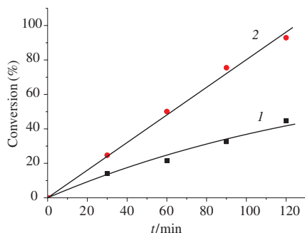
Figure 1 Conversion of 1d in the presence of AHSs (1) 3g /Amb and (2) 3h /Amb. [ 1d ] = 0.01 mol dm -3 , LEDs, MeCN–H 2 O (1:1), \alpha = 3950, selectivity towards 2d > 90%.
