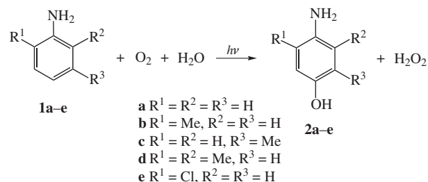
Scheme 1 Reagents and conditions: PcM, MeCN–H 2 O, 25 °C, visible light irradiation.
