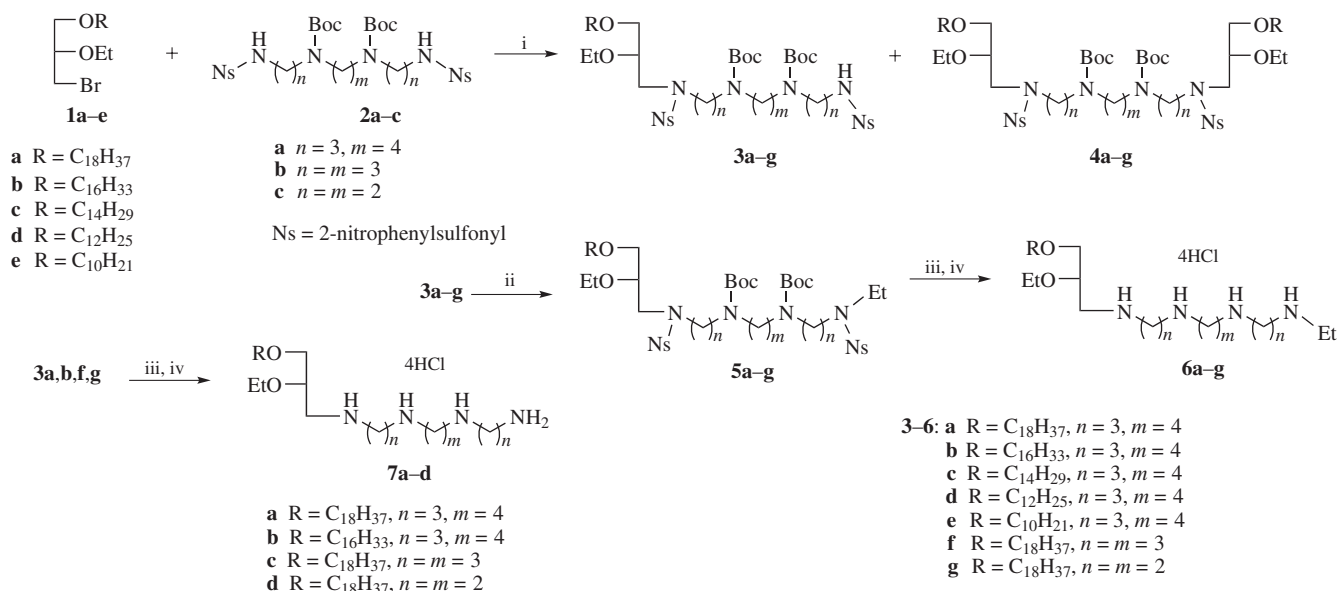
Scheme 1 Reagents and conditions: i, Cs 2 CO 3 , DMF, 85 °C; ii, EtBr, Cs 2 CO 3 , DMF, 85 °C; iii, PhSH, K 2 CO 3 , 24 °C; iv, 4 N HCl-dioxane, 24 °C.
