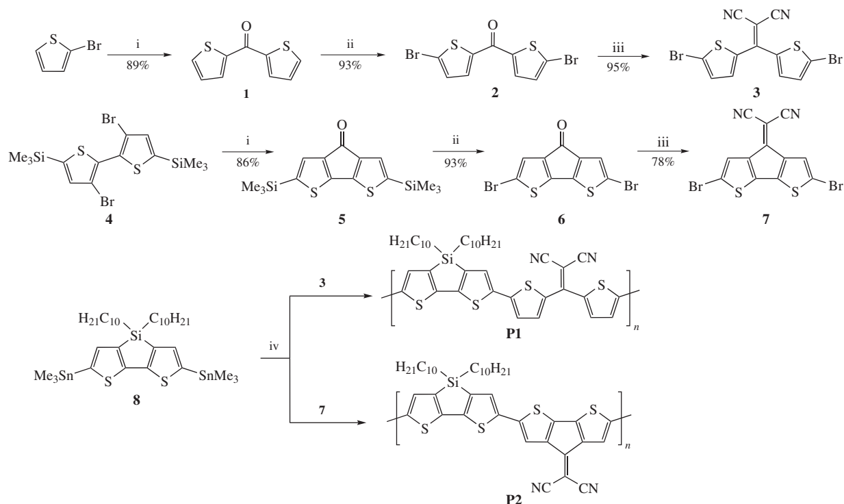
Scheme 1 Reagents and conditions: i, \text{Bu}^n\text{Li} , THF, -78^\circ\text{C} , then \text{Me}_2\text{NC(O)Cl} ; ii, NBS, DMF; iii, \text{CH}_2(\text{CN})_2 , pyridine; iv, \text{Pd(PPh}_3)_4 , toluene, reflux.
