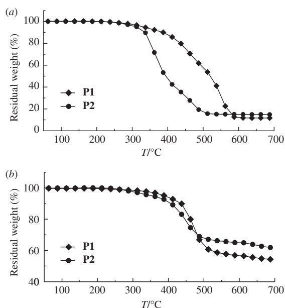
Figure 1 TGA curves of the copolymers measured in (a) air and (b) nitrogen.
