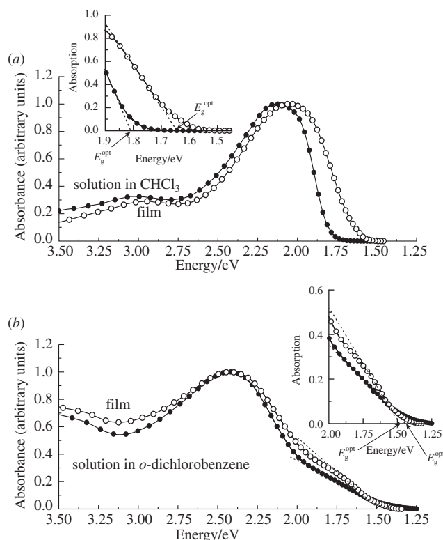
Figure 2 UV-VIS spectra of copolymers (a) P1 and (b) P2 obtained in solutions and in thin films. Sidebars show methods of determination the E_g using edges of the absorption spectra.
