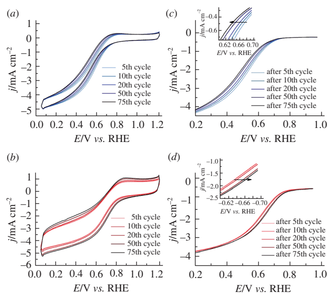
Figure 3 CV curves for (a) CoZ-68-C and (b) CoZ-69-C collected in 0.1 M \text{HClO}_4 at a scan rate of 20 \text{mV s}^{-1} , 25 ^\circ\text{C} in an \text{O}_2 atmosphere at a rotation rate of 1600 rpm and the LSV curves for (c) CoZ-68-C and (d) CoZ-69-C.
