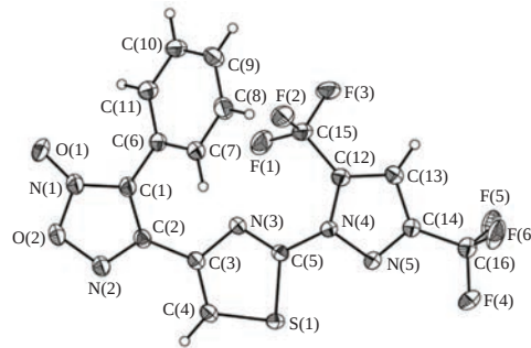
Figure 1 ORTEP view of the molecular structure of 4f with thermal ellipsoids drawn at the 50% probability level.
