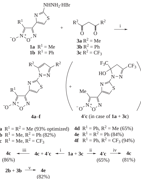
Scheme 3 Reagents and conditions: i, AcOH, 0.35 equiv. H 2 SO 4 , 80 °C, 6 h; ii, EtOH, 0.35 equiv. H 2 SO 4 , 80 °C, 5 h; iii, AcOH, 0.35 equiv. H 2 SO 4 , 80 °C, 11 h; iv, AcOH, 1.0 equiv. H 2 SO 4 , 80 °C, 5 h; v, AcOH, 0.35 equiv. H 2 SO 4 , 80 °C, 6 h. Molar ratios: 1 : 3a,c = 1:2, 1 : 3b = 1:1.4.
