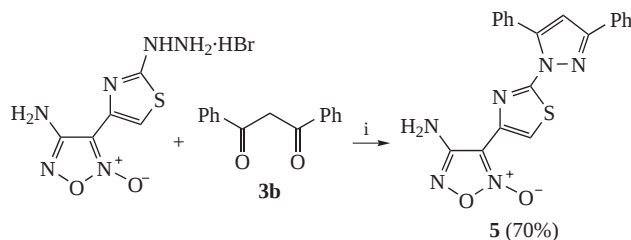
Scheme 4 Reagents and conditions: i, AcOH, 0.35 equiv. H 2 SO 4 , 80 °C, 6 h.
