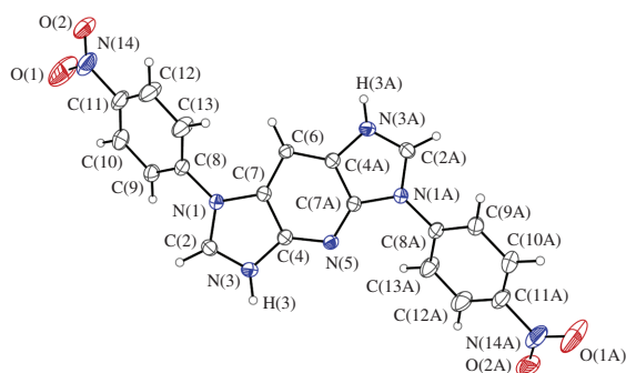
Figure 3 General view of the cation of 7b in thermal ellipsoid representation ( p = 50\% ). Only one part of the overlapping pseudo-centrosymmetric heterocycles is shown. The trifluoroacetate anions and trifluoroacetic acid solvate molecules are omitted for clarity.
