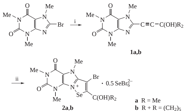
Scheme 1 Reagents and conditions: i, HC≡CC(OH)R 2 , [Pd], PhMe–NMP; ii, SeO 2 , conc. HBr, dioxane, ~20 °C, 24 h.
