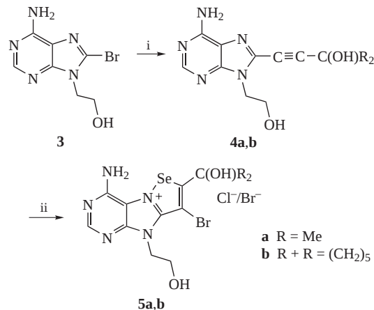
Scheme 2 Reagents and conditions: i, HC≡CC(OH)R 2 , (Ph 3 P) 2 PdCl 2 , CuI, DMF, Et 3 N, ~20 °C, 18 h; ii, SeO 2 , conc. HBr, dioxane, ~20 °C, 24 h, then ion-exchange (Cl − ) resin.
