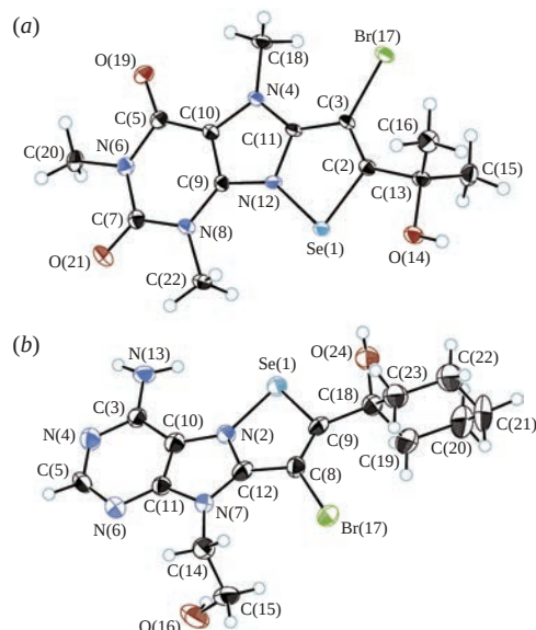
Figure 1 ORTEP diagram of cations of compounds (a) 2a and (b) 5b with atomic labels and thermal ellipsoids (50%).
