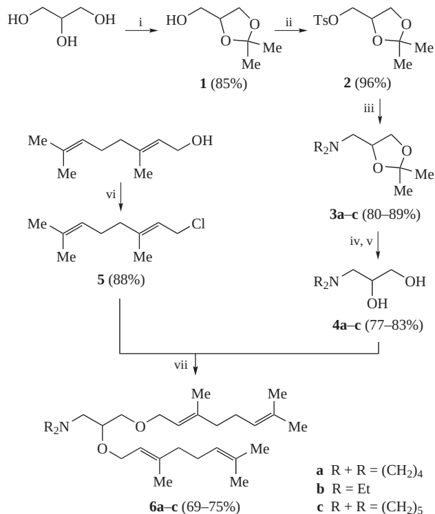
Scheme 1 Reagents and conditions: i, Me 2 CO, TsOH, room temperature; ii, TsCl, pyridine, room temperature; iii, R 2 NH, 100 °C; iv, 1 M HCl, room temperature; v, MeONa, MeOH, room temperature; vi, CCl 4 , PPh 3 , reflux; vii, NaH, abs. THF, reflux.
