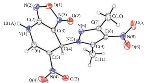
Figure 1 General view of molecule 4d in crystal. Anisotropic displacement parameters are drawn with 50% probability, only the major component of the disordered heterocyclic moiety is shown.
