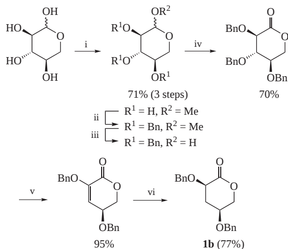
Scheme 3 Reagents and conditions: i, SOCl 2 , MeOH, reflux; ii, NaH, BnBr, THF, DMF; iii, H 2 SO 4 , H 2 O, 1,4-dioxane, AcOH, reflux; iv, I 2 , K 2 CO 3 , CH 2 Cl 2 ; v, TBD, 130 °C; vi, H 2 , PtO 2 , AcOEt.
