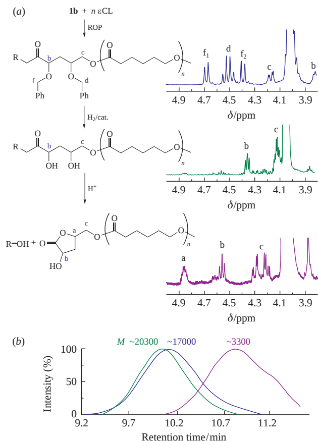
Figure 2 (a) The scheme of the synthesis and degradation of polymer 4b and the corresponding fragments of ^1\text{H} NMR spectra and (b) SEC traces.
