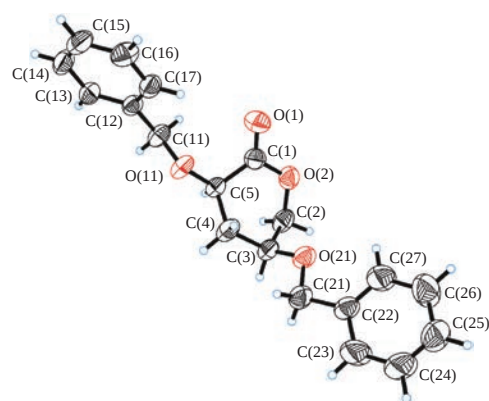
Figure 1 Molecular structure of 2,4-dibenzyloxy- \delta -valerolactone 1b (50% thermal ellipsoid probability). Selected bond lengths (Å): C(1)–O(1) 1.192(2), C(1)–O(2) 1.349(2), C(1)–C(5) 1.512(2), C(2)–O(2) 1.442(2), C(2)–C(3) 1.503(2), C(3)–C(4) 1.533(2), C(4)–C(5) 1.5200(19).
