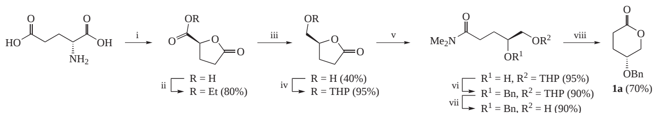
Scheme 2 Reagents and conditions: i, NaNO 2 , H 2 SO 4 ; ii, EtOH, TsOH; iii, NaBH 2 , EtOH; iv, THP, CH 2 Cl 2 ; v, Me 2 NH, H 2 O; vi, BnBr, NaH, THF; vii, TsOH, MeOH; viii, TsOH, C 6 H 6 , reflux.
