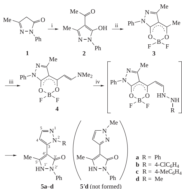
Scheme 1 Reagents and conditions: i, MeC(OEt) 3 , then AcOH–H 2 O, Δ; ii, B(OBu) 3 , BF 3 ·OEt 2 ; iii, Me 2 NCH(OMe) 2 ; iv, RNHNH 2 .
