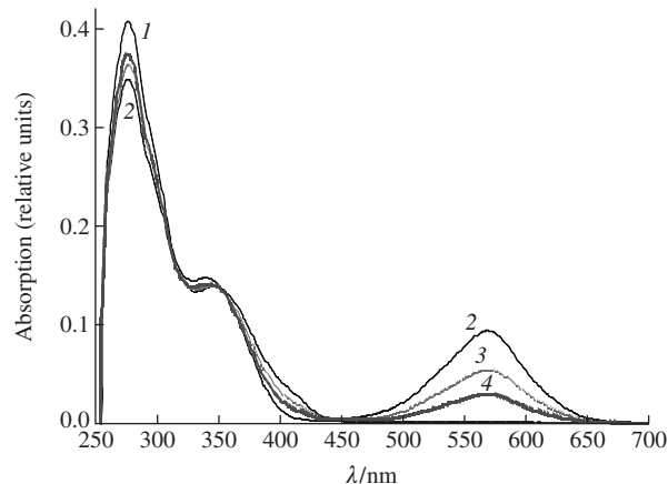
Figure 3 Absorption spectra of compound 4 in DMSO, 25 °C: (1) original solution, (2) after UV illumination at 365 nm (3) after subsequent storage in the dark for 1 min and (4) after subsequent storage in the dark for 5 min.
