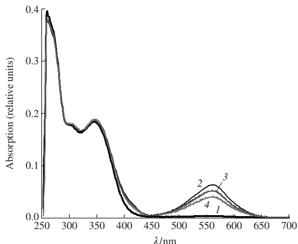
Figure 2 Absorption spectra of compound 2 in DMSO, 25 °C: (1) original solution, (2) after UV illumination at 365 nm, (3) after subsequent storage in the dark for 3 min and (4) after subsequent storage in the dark for 10 min.
