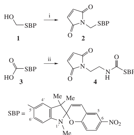
Scheme 1 Reagents and conditions: i, PPh 3 , DIAD, neopentyl alcohol, maleimide, THF, –70 °C; ii, HBTU, N-(2-aminoethyl)maleimide, TFA, N-methylmorpholine, DMF, 0 °C.
