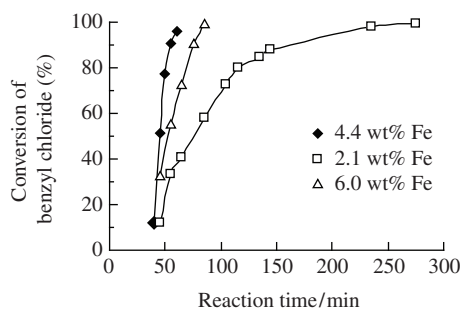
Figure 3 Conversion of benzyl chloride in the benzylation of benzene at 60 °C over the FS400 catalysts with different iron contents.
