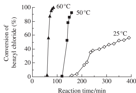
Figure 1 Effect of reaction temperature on the conversion of benzyl chloride in the benzylation of benzene over the 4FS400 catalyst.
