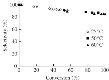
Figure 2 Selectivity for diphenylmethane formation as a function of benzyl chloride conversion over the 4FS400 catalyst.
