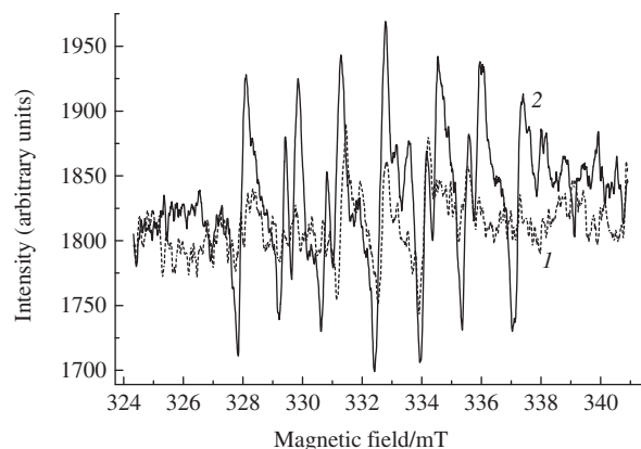
Figure 2 ESR spectra of (1) P(OEt)_3 –DMPO (weak signal due to some impurity is visible) and (2) the reaction mixture P(OEt)_3 + DMPO + C_{70}Cl_{10} in toluene.
