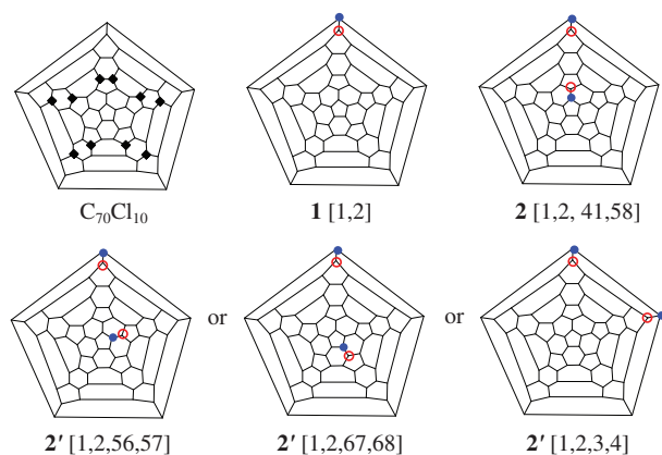
Figure 1 Schlegel diagrams of C_{70}Cl_{10} , products 1 , 2 and possible molecular structures of minor component 2' . Filled circles denote H, opened circles denote P(O)(OEt)_2 , and filled diamonds denote Cl.
