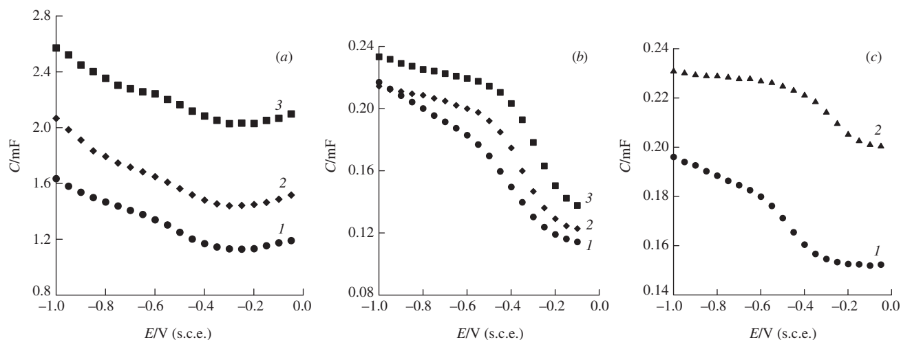
Figure 1 C(E) curves on a nanopaper electrode (a) in (1) 0.1 M \text{Na}_2\text{SO}_4 , (2) 0.1 M \text{Na}_2\text{SO}_4 + 10^{-4} M camphor and (3) 0.1 M \text{Na}_2\text{SO}_4 + 10^{-3} M camphor solutions; (b) in (1) 0.1 M \text{Na}_2\text{SO}_4 , (2) 0.1 M \text{Na}_2\text{SO}_4 + 10^{-4} M sodium cryptate and (3) 0.1 M \text{Na}_2\text{SO}_4 + 10^{-3} M sodium cryptate solutions; (c) in (1) 0.01 M \text{MgSO}_4 and (2) 0.01 M \text{MgSO}_4 + 10^{-2} M cryptofix solutions. Surfaces of electrodes are different for (a), (b) and (c).
